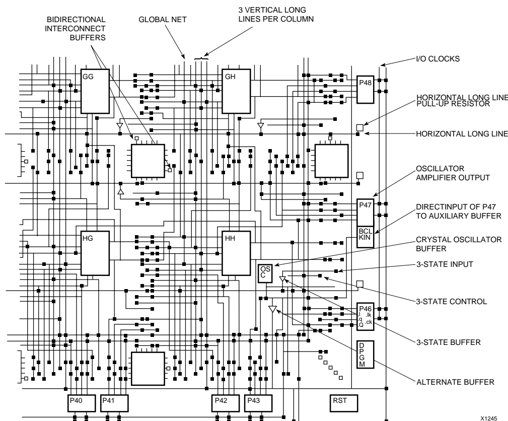
Figure 18: Design Editor.
